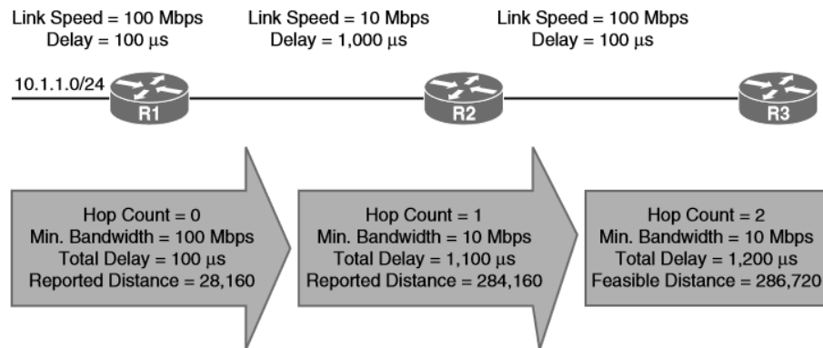
Figure 2-9 EIGRP Attribute Propagation
