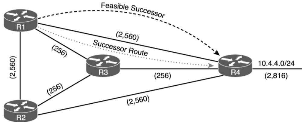
Figure 2-2 EIGRP Reference Topology
